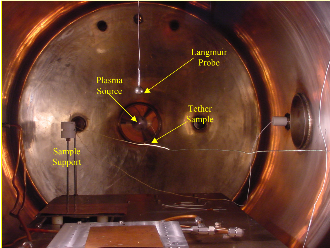
Figure 2. ProSEDS High Voltage Plasma Interactions Internal Chamber Set-Up
