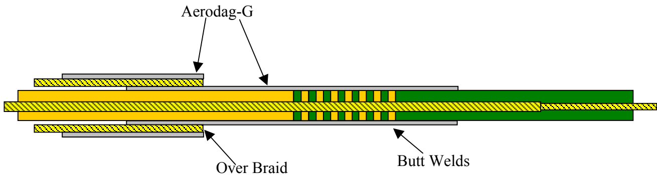
Figure 7. ProSEDS Tether Triple Point Mitigation Design
