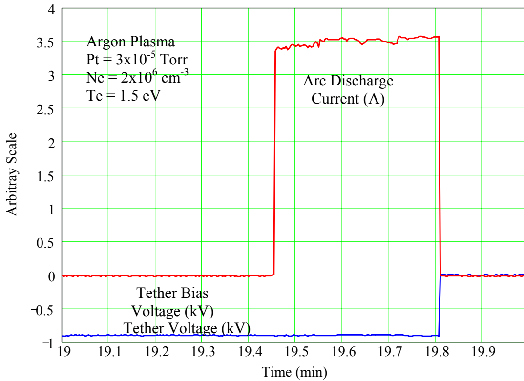
Figure 5. Current and Voltage Data Due to ProSEDS Conductive Tether Triple Point Discharge
