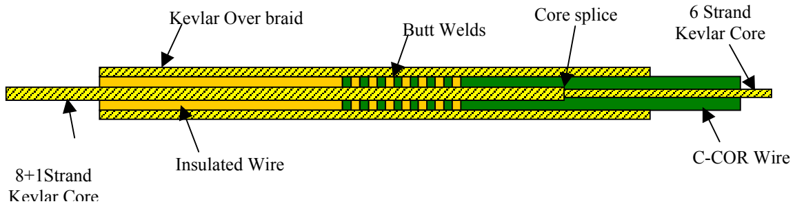
Figure 4. ProSEDS as Designed Conductive Tether to Insulated Transition
