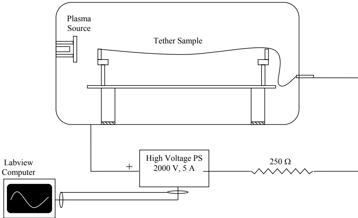
Figure 3. Tether High Voltage Test Schematic
